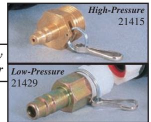
Constant-flow Connector
